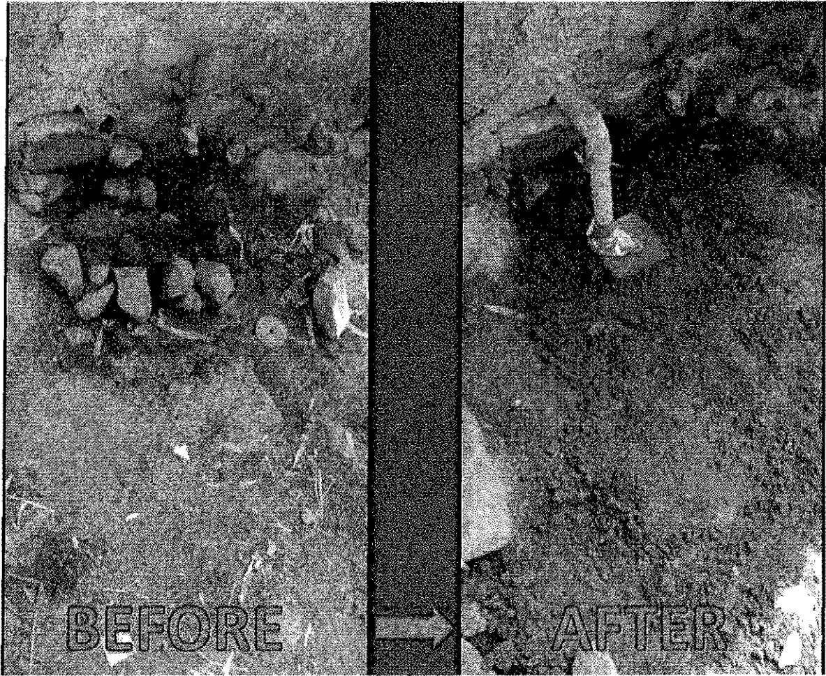
Soak-pit Construction Work
